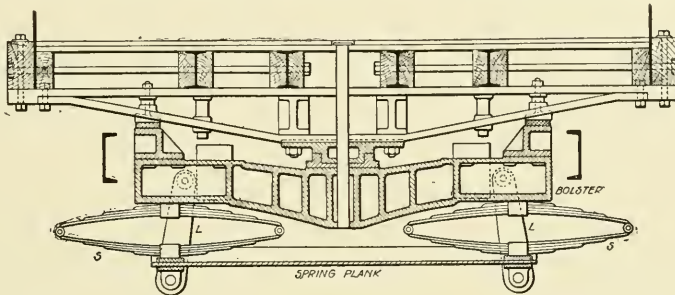
Fig. 11. Section of Bolster, Elliptical Springs and Spring Plank
